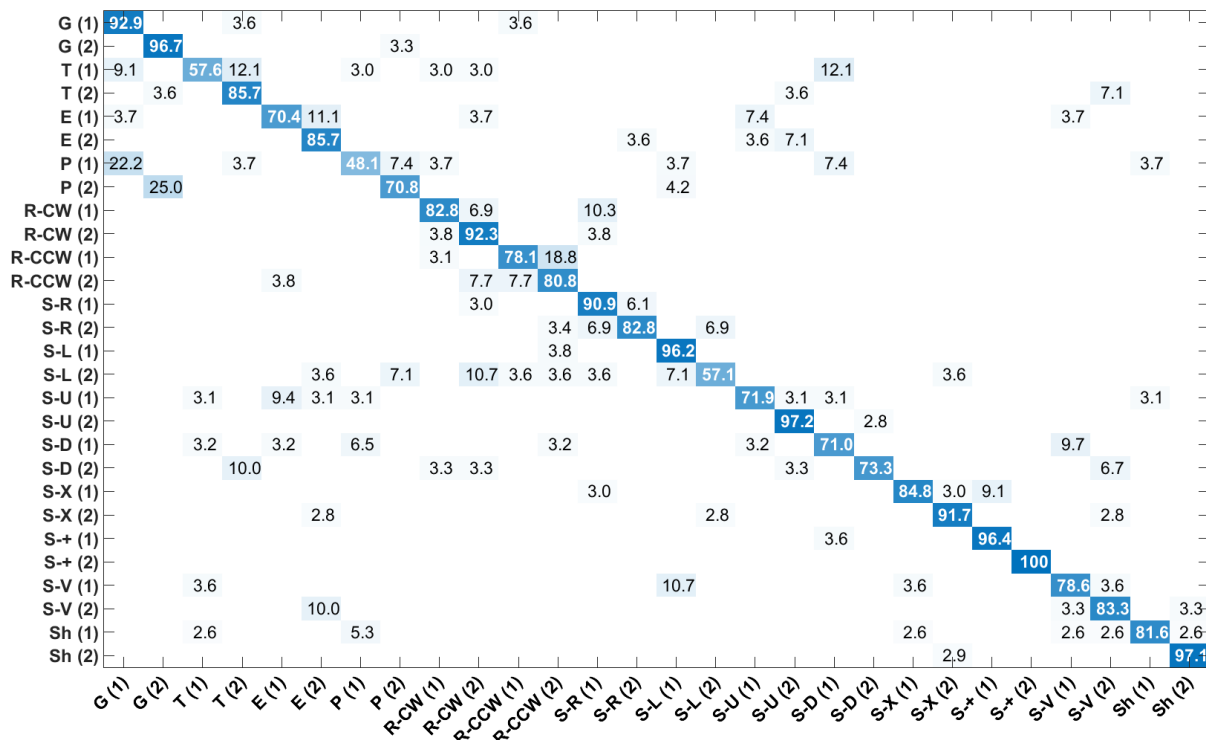
Figure 7: Confusion matrix (28 gesture classes) obtained by De Smedt et al. [DSWVI6].
