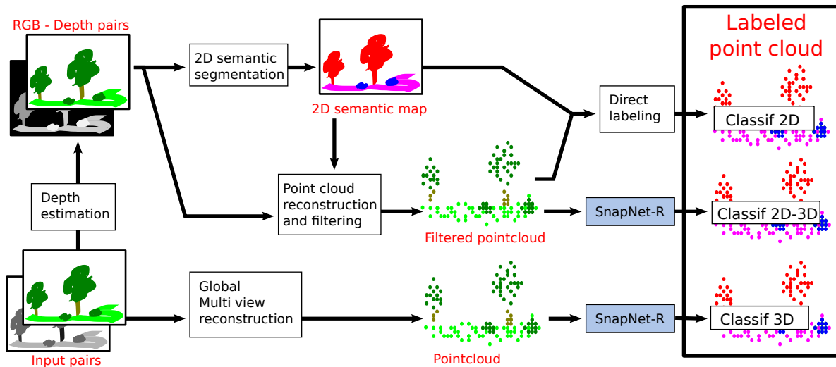
Pipelines and processing blocks are described in section 3.3. Qualitative results on 3DRMS are discussed in section 4.4. Figure 3. 3D reconstruction and labeling pipelines for the 3DRMS challenge.
